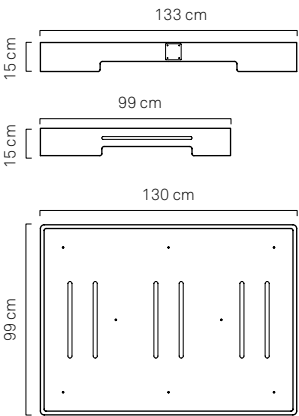
BASAMENTO MAGNUM / MAGNUM PLEXI BASE
