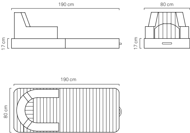
POLTRONA APERTA / OPENED ARMCHAIR
