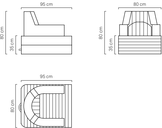
POLTRONA CHIUSA / CLOSED ARMCHAIR
